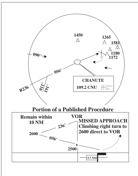
FIG 5-4-32 Missed Approach
