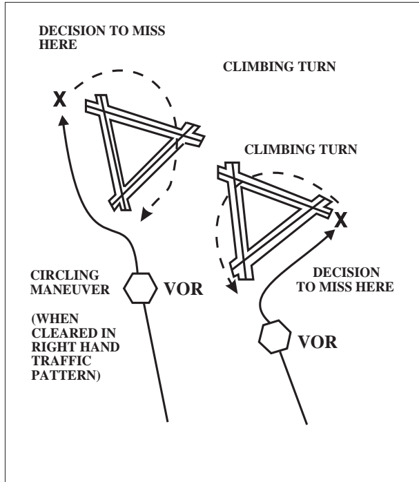
FIG 5-4-31 Circling and Missed Approach Obstruction Clearance Areas
