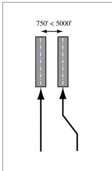
FIG 5-4-26
